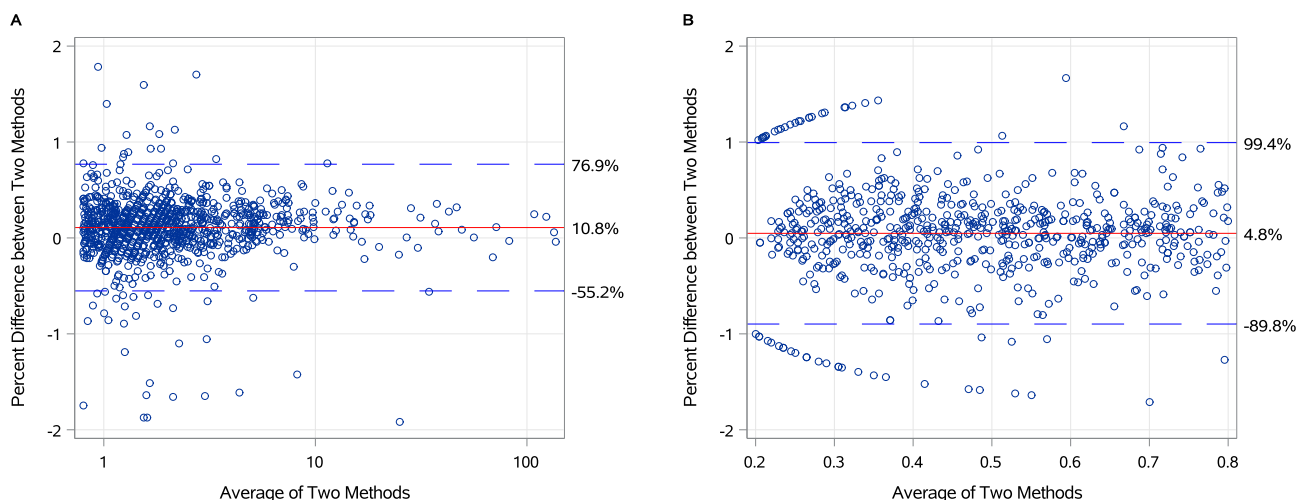
Fig. 4. Bland-Altman analysis of percentage differences stratified according to values equal to or above LOQ ( \geq 0.8 \mu\text{g/mL} ) with \times axis in log-10 scale (panel A) and values between the LOD and LOQ (panel B) ( 0.2 - < 0.8 \mu\text{g/mL} ).
